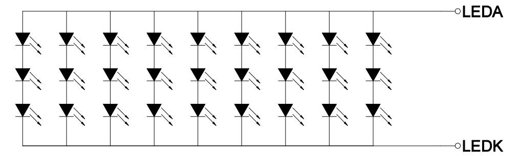
LED Diagram Circuit
