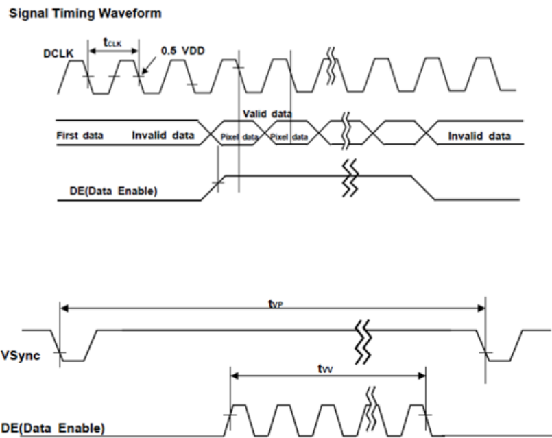
Figure 8. Signal Timing Waveform
