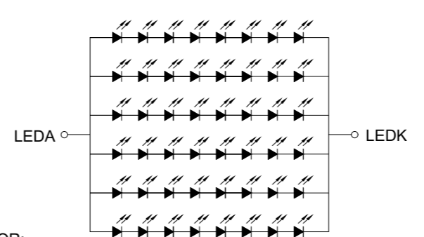
LED Diagram Circuit
