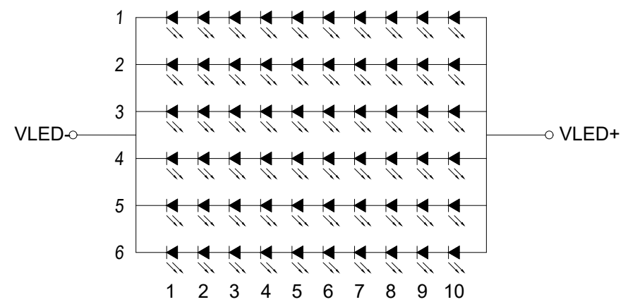
LED Diagram Circuit
